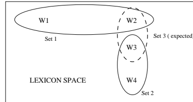
Figure 1: Example for the clustering problem of greedy algorithm in a lexicon space with four different words. Note that d_{w_2, w_3} is the smallest distance in the distribution. However since w_1 is taken into consideration, it forms set 1 with its nearest neighbor w_2 and w_3 combines with w_4 and form set2, although w_2 is nearer. And the expected third set is not formed.
