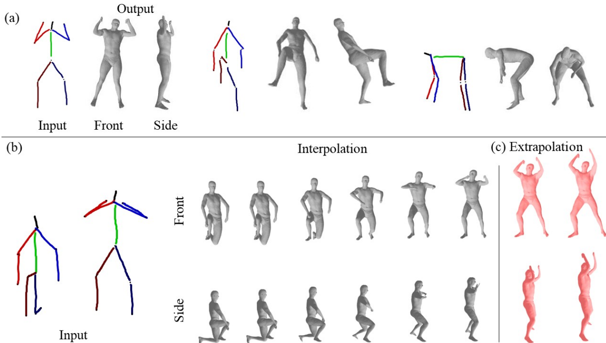
Figure 1: Our framework is capable of performing three tasks. (a) It can generate 3D models from given 2D stick figure sketches. (b) It can generate dynamic 3D models, i.e., animations, between given source and target stick figures. (c) It can further extrapolate the produced 3D model sequence by using the learned interpolation vector.
