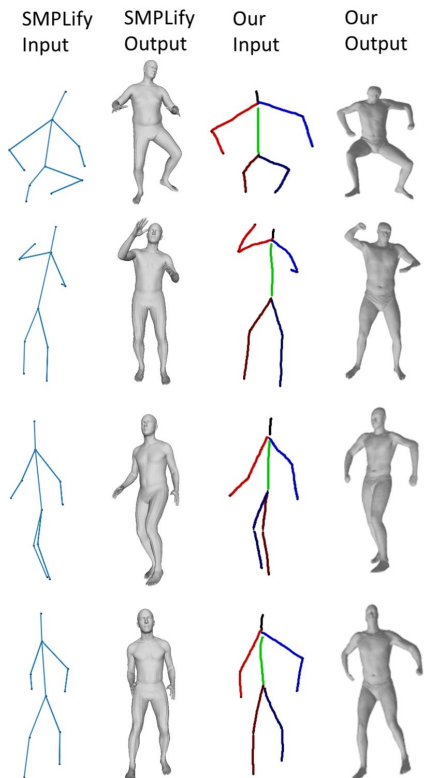
Figure 6: Qualitative comparison of our method (columns 3 and 4) with [20] (columns 1 and 2).
