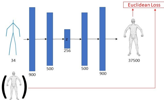
Figure 4: Neural network architecture for standard autoencoder baseline.
