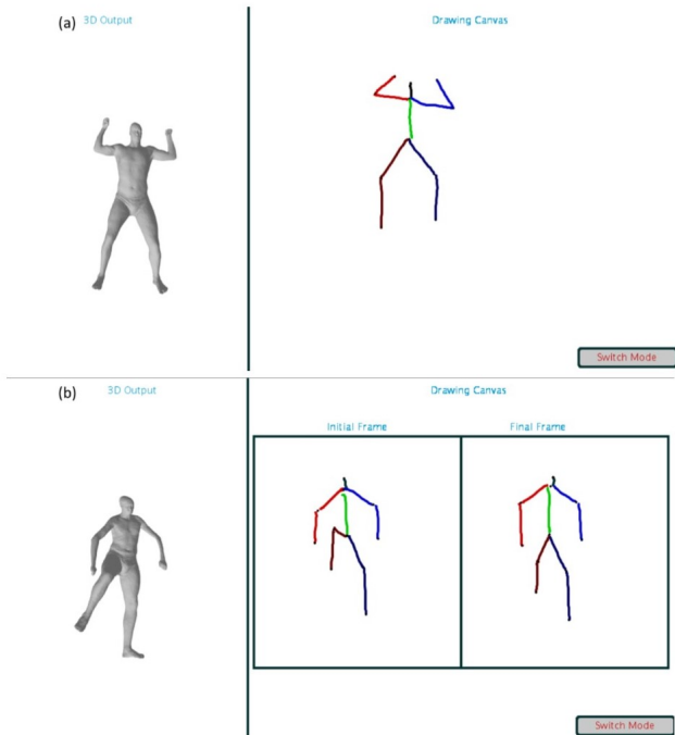
Figure 3: Screenshots from our user interface. (a) 3D model generation mode. (b) 3D animation generation mode.
