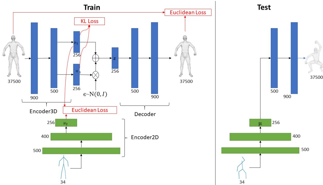
Figure 2: Our neural network architecture. (a) Train Network: We train this network with (3D point cloud, 2D points of stick figure) pairs during training time. It consists of a VAE: Encoder3D and Decoder consecutively, and another external encoder: Encoder2D. We use regression loss from the output of Encoder2D to the mean vector of the VAE in addition to standard losses of VAE. (b) Test Network: We remove Encoder3D and reparameterization layer from our VAE and use Encoder2D-Decoder as our network in our experiments.
